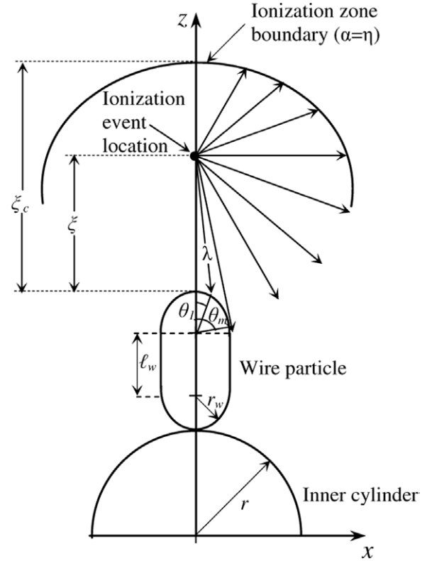
Figure A1. Propagation of photon in the ionization zone in radial directions from an ionization event along the route of the avalanche.
